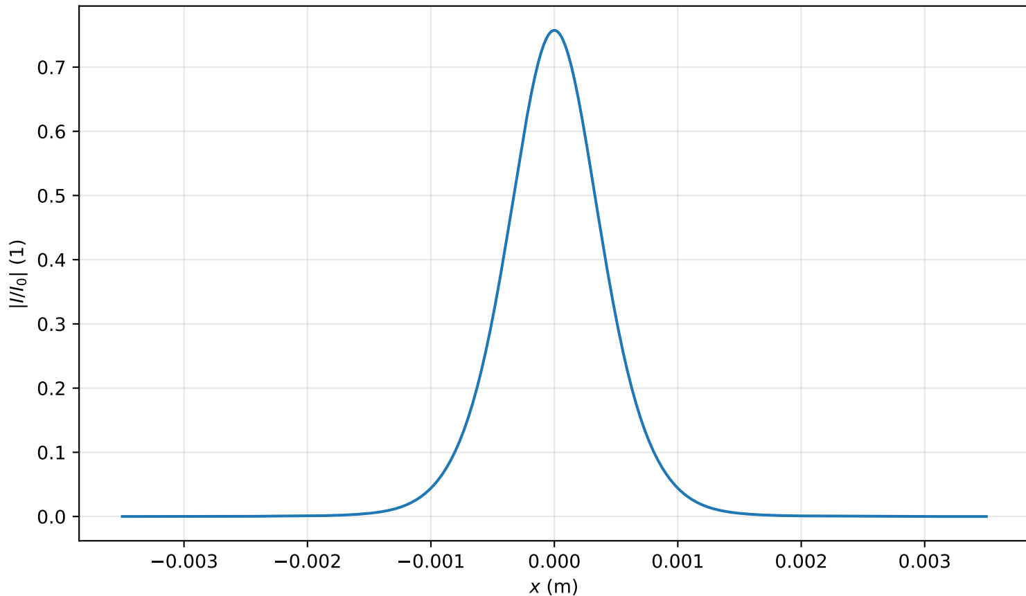
Intensity profile I(x, y = 0, z = 3.344m)/I_0 , P_{in}=0.7P_{cr} , artificial time
